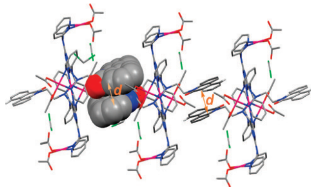
Figure 2. Perspective view showing the one-dimensional supramolecular chains assembled by means of \pi - \pi stacking interactions. The mean distance d between the two phenanthridine planes amounts to 3.391 Å.
