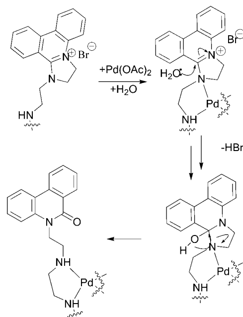
Scheme 3. Proposed Mechanism for the Ligand Transformation upon Coordination of Compound 3 by \text{Pd}(\text{OAc})_2
