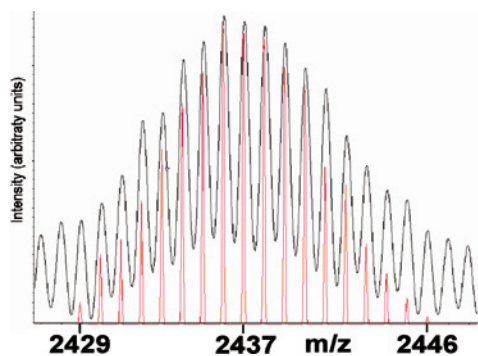
Figure 3. Cryospray mass spectrum (negative ion mode) of compound 4 in a DCM/MeCN (1:1) mixture at -40\text{ }^{\circ}\text{C} shown in black. The simulated spectrum for [\text{Pd}_5(\text{C}_{40}\text{H}_{34}\text{N}_{12}\text{O})_2(\text{CH}_3\text{CO}_2)_5\text{Cl}_6]^- is shown in red.
