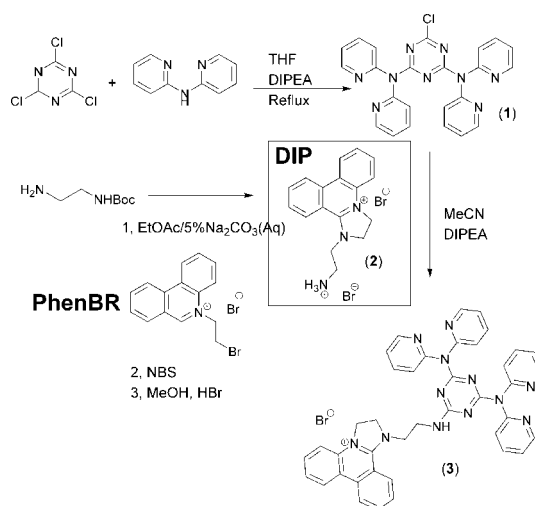
Scheme 1. Synthesis of Compound 3 a
