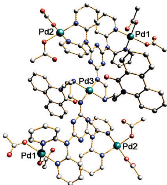
Figure 1. Ball-and-stick representation of [\text{Pd}_5(\text{L})_2(\text{OAc})_8]^{2+} . The solvent and anions of crystallization, as well as the H atoms, are omitted for clarity: C, gray; N, blue; O, red; Pd, green. Pd3 rests on an inversion center.
